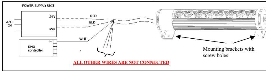
Figure 2: Single Color Dimmable LP Fixture
