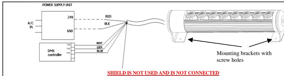
Figure 3: TRI COLOR (RGB) Dimmable LP Fixture
