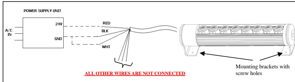
Figure 1: Single Color Non-Dim LP Fixture
